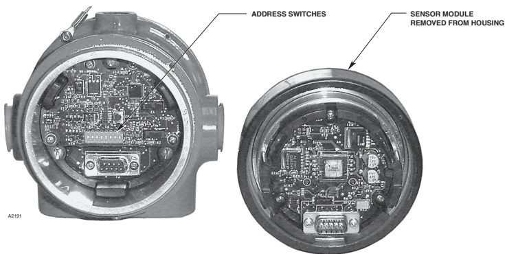
Figure 17—Location of Address Switches
