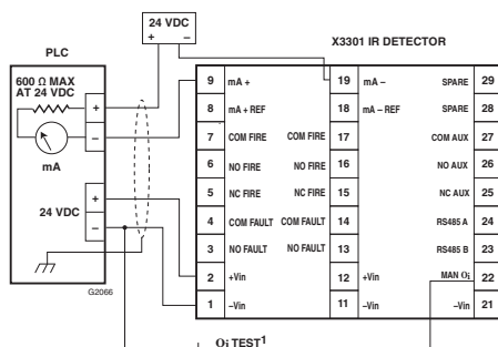
Figure 13—X3301 Detector Wired for Isolated 0 to 20 mA Current Output (Sinking)
