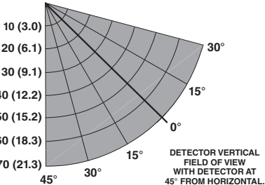
Field of View at Indicated Distance in Feet (m) for Isopropanol at Very High Sensitivity (6 in. x 6 in.)
