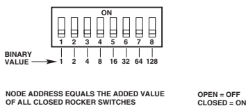
Figure 18—Address Switches for X3301
