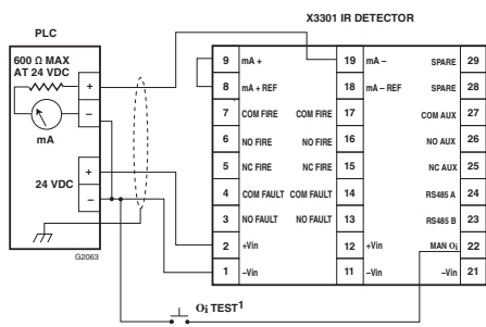
Figure 10—X3301 Detector Wired for Non-Isolated 0 to 20 mA Current Output (Sourcing)
