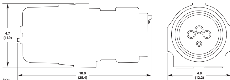
Figure 20—X3301 Dimensions in Inches (cm)
