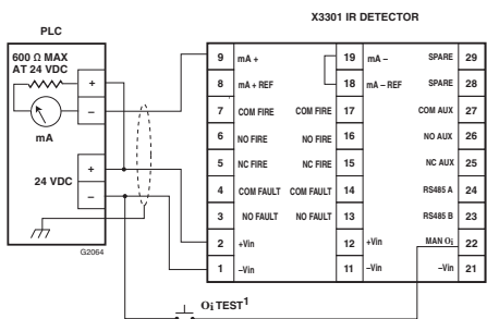
Figure 12—X3301 Detector Wired for Non-Isolated 0 to 20 mA Current Output (Sinking)
